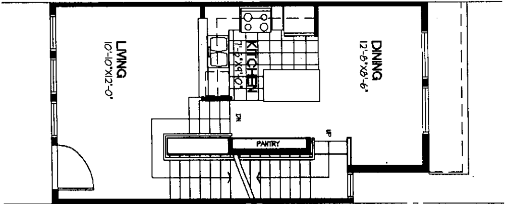
2nd FLOOR PLAN AREA = 480.7 SF
