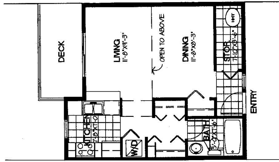
1ST FLOOR PLAN AREA = 475.8 SF
