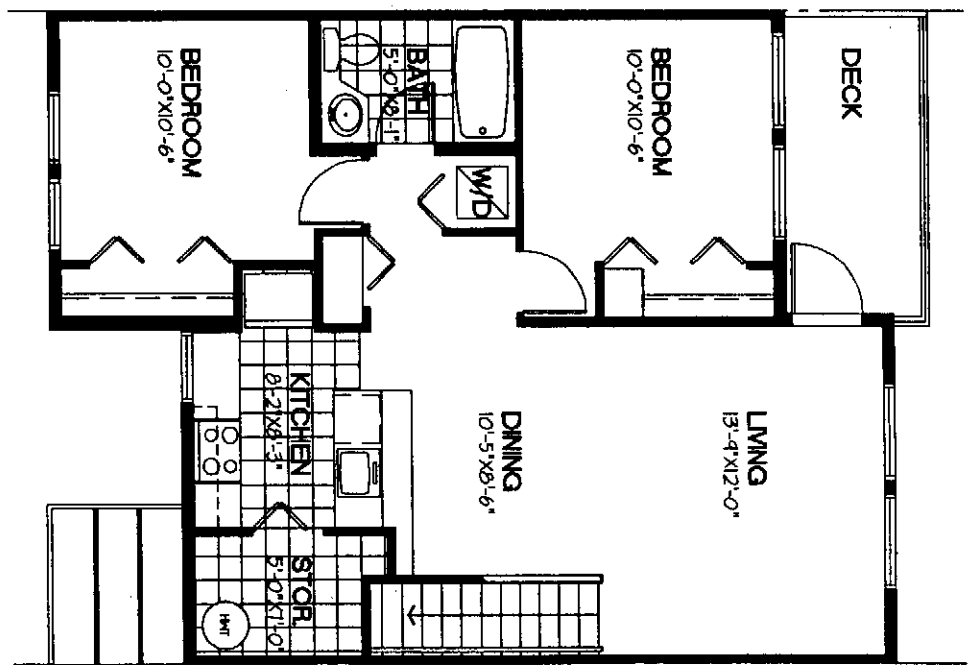
2 BEDROOM FLAT AREA = 833.0 SF (+ 85.5 SF @ GROUND FLOOR) (TOTAL AREA = 918.5 SF)
